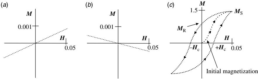
Figure 8.2. Different types of magnetic behavior: (a) a typical M–H curve (both axes in Teslas) of a paramagnetic substance; (b) a diamagnetic substance; and (c) a ferromagnetic substance (note the change in the scale of the M axis). An isotropic single crystal, or polycrystal with random crystallite orientation, is assumed.
