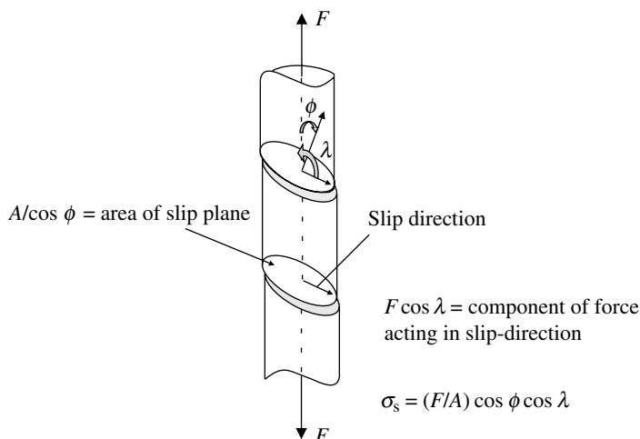
Figure 10.6. Application of a tensile force to a cylindrical single crystal causes a shear stress on some crystal planes. When the shear stress is equal to the critical-resolved shear stress (the yield stress), glide proceeds along the slip direction of the planes.
