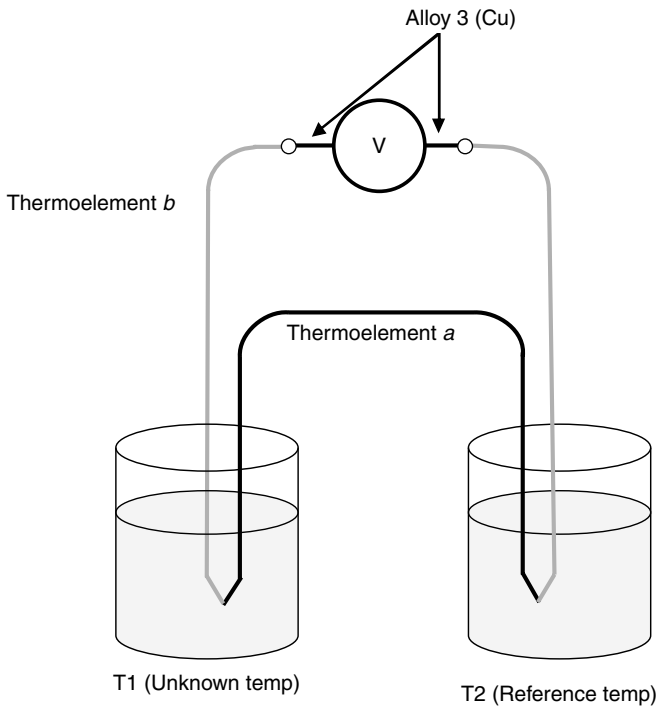
Figure 6.3. A schematic diagram illustrating the generation of a TE voltage.
