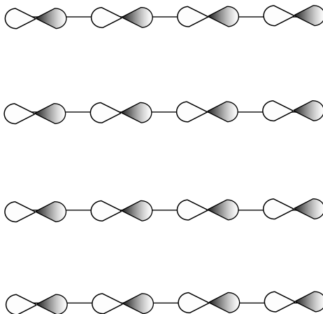
Figure 5.2. A two-dimensional square array of p_x atomic orbitals. The bonding is by \sigma interactions in the horizontal direction and by \pi interactions in the vertical direction.
