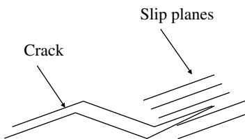
Figure 10.14. The single-slip mechanism, in which crack growth occurs in the direction of the primary slip systems, results in a zig-zag crack path.
