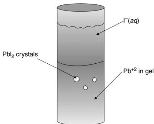
Figure 12.4. Gel growth of single crystalline \text{PbI}_2(\text{s}) .
