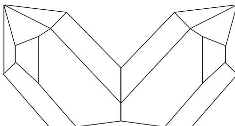
Figure 1.14. A drawing of a Japan-Law contact twin quartz crystal. This type of twinning was first discovered in 1829 by C. S. Weiss in quartz crystal from the La Gardette mine in France. However, because of the abundance of these specimens in Japan, they are now known as Japanese twins.
