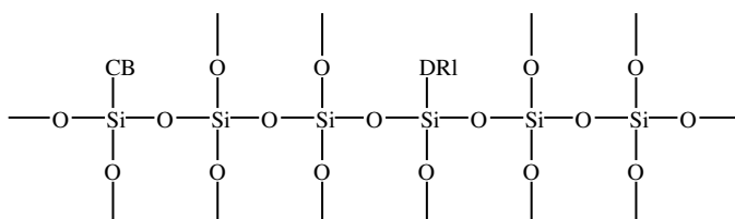
Figure 12.7. Spacing of CB and DR1 on a \text{SiO}_2 backbone.
