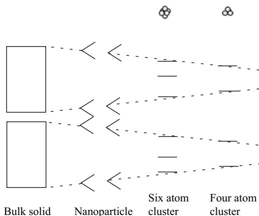
Figure 13.1. The particle size regime at which a gradual transition occurs from quasi-continuous energy bands to experimentally observe discrete energy levels fall somewhere in the nanoscale range.
