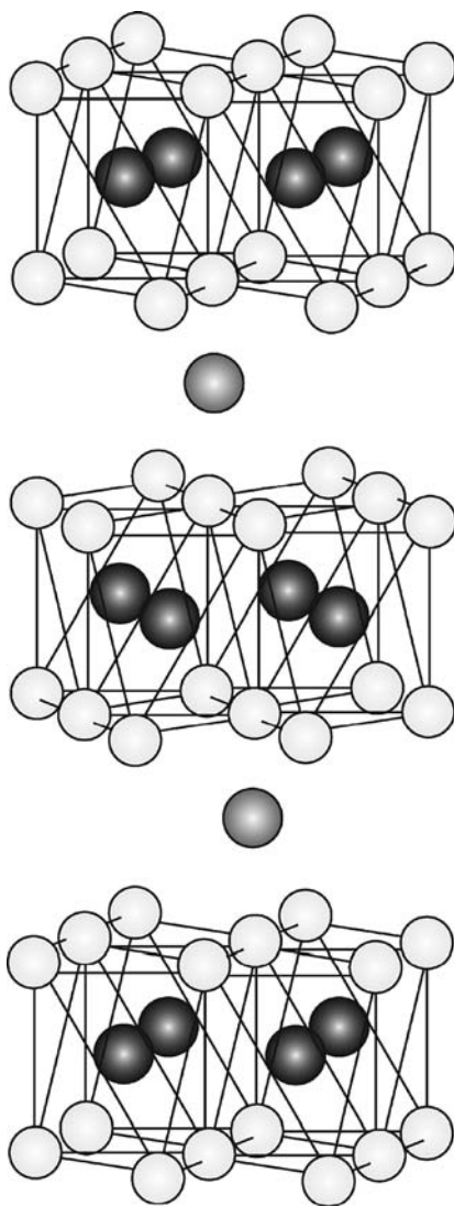
Figure 3.16. The hexagonal delafossite structure. Lightly shaded circles are oxygen atoms. The dark circles in the centers of the octahedra are the B atoms. The A atoms are the gray circles located between the slabs of edge-sharing BO_6 octahedra.
