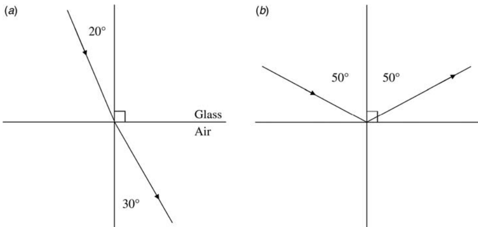
Figure 9.4. Refraction (a) versus total internal reflection (b).
