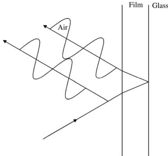
Figure 9.9. Reflections from front and back surface of thin film.
