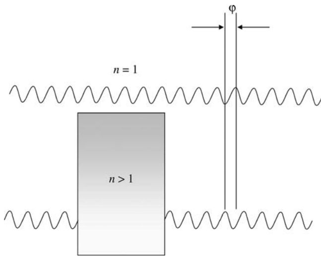
Figure 9.6. Phase shift ( N ) of light passing through refractive index n .
