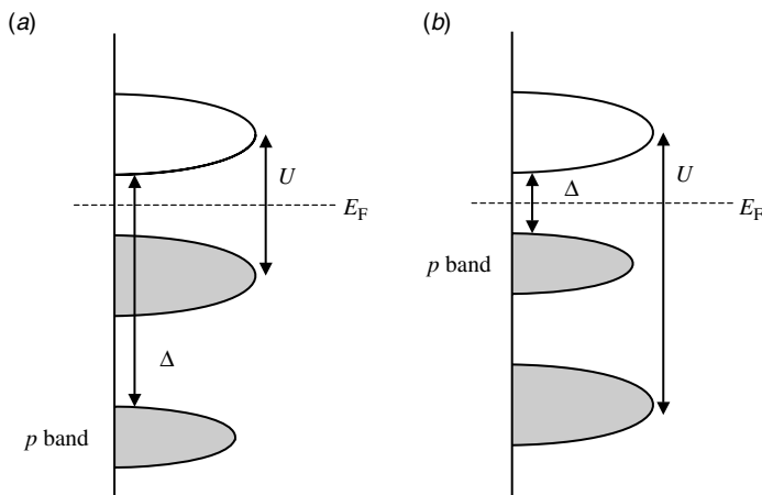
Figure 7.1. The band gap is determined by the d-d electron correlation in the Mott–Hubbard insulator (a), where \Delta > U . By contrast, the band gap is determined by the charge transfer excitation energy in the charge transfer insulator (b), where U > \Delta .
