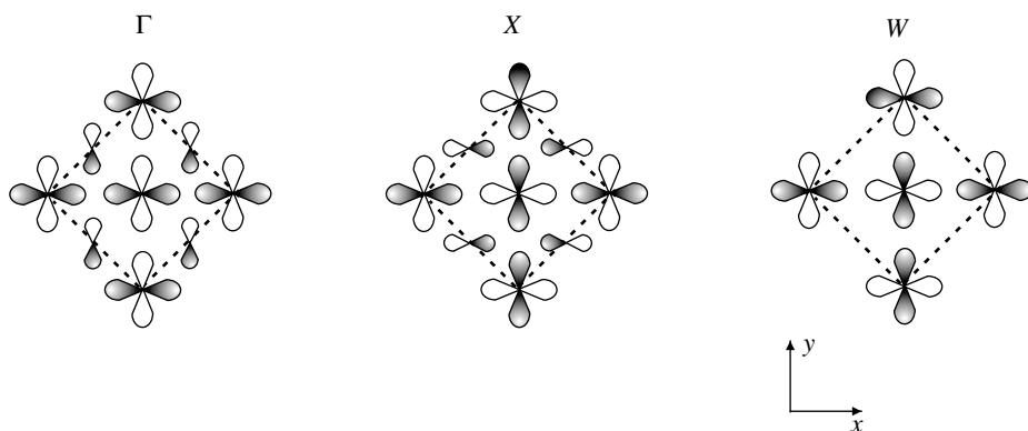
Figure 5.16. The d_{x^2-y^2} - d_{x^2-y^2} and p - d interactions at \Gamma , X , and W , in the transition metal monoxides with the rock-salt structure, viewed down [001] .
