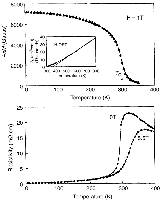
Figure 8.7. Example of experimental data on a CMR material. The ferromagnetic Curie temperature for \text{La}_{0.65}(\text{CaPb})_{0.35}\text{MnO}_3 is slightly higher than the NM–M transition temperature. (After Pickett and Singh (1996). © American Institute of Physics. Reproduced with permission.)
