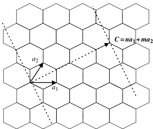
Figure 5.4. The chiral vector, \mathbf{C} , defines the location of the two lattice points that are connected to form a nanotube.
