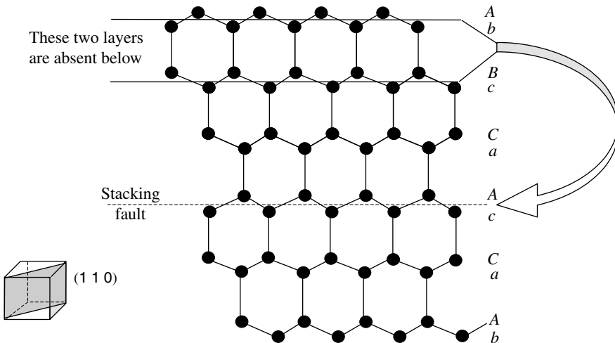
Figure 2.7. A (1 1 0) section through a diamond lattice showing a stacking fault by the absence of two adjacent atomic layers. The layer-sequence along the \langle 1\ 1\ 1 \rangle body-diagonal direction should be \dots AbBcCaAb\dots .
