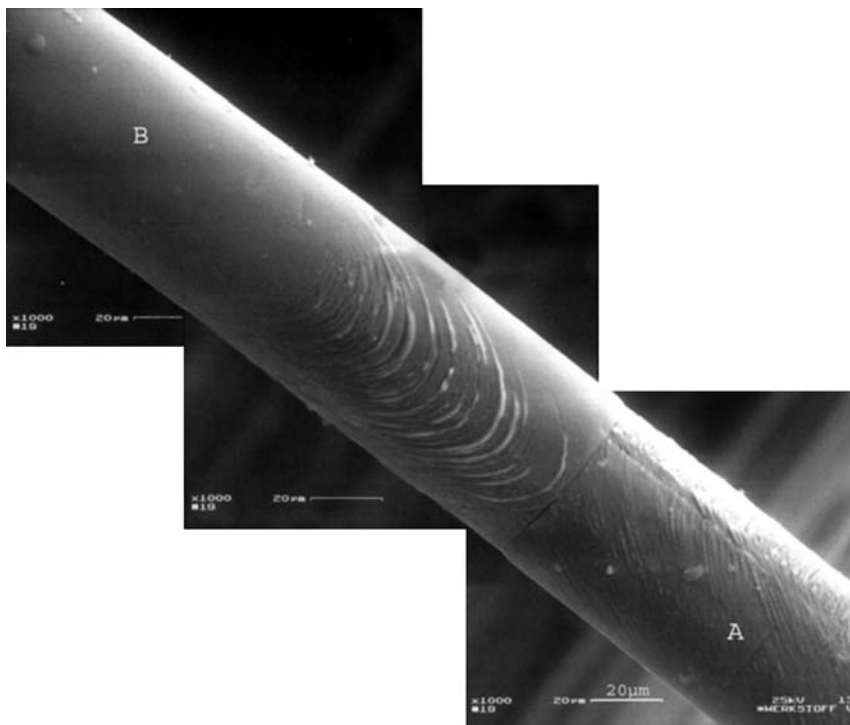
Figure 10.10. Slip-band formation on the surface of a fatigued bamboo structured copper wire of 50 \mu\text{m} diameter. (From G. Khatibi, A. Betzwar-Kotas, V. Gröger, and B. Weiss, A Study of the Mechanical and Fatigue Properties of Metallic Microwires , Fatigue & Fracture of Engineering Materials & Structures , Vol. 28, No. 8, pp. 723–733, (2005). Reproduced with permission.)
