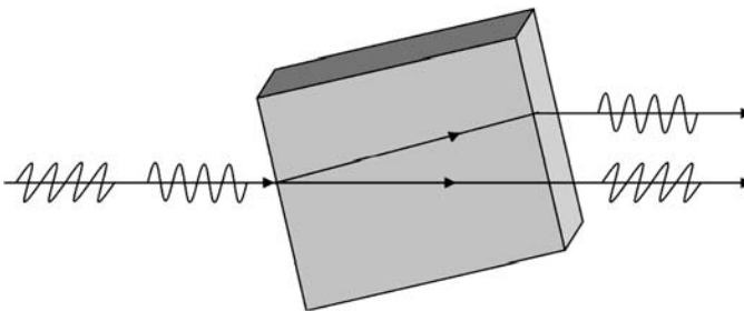
Figure 9.3. Physical separation of a light beam into its two polarizations.
