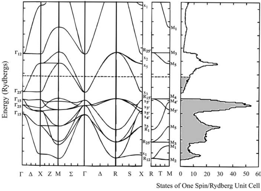
Figure 4.7. The LCAO (tight-binding) band structure for \text{ReO}_3 . The dashed line represents the Fermi energy. To the far right is the density-of-states (DOS) curve for states of one spin. The occupied states (up to the Fermi level) are shaded gray. Note that the valence band is completely filled while the conduction band is partially filled. Hence, \text{ReO}_3 should be metallic.
