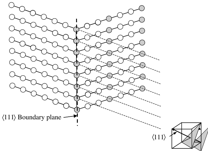
Figure 1.16. The twin boundary (perpendicular to the plane of the page) is a \Sigma 3 misorientation. Note that there is complete coincidence in the boundary plane itself.
