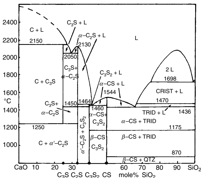
Figure 11.9. The \text{CaO-SiO}_2 phase diagram at one atm pressure. (After West, Solid State Chemistry and its Applications , 1985. © John Wiley & Sons, Inc. Reproduced with permission.)
