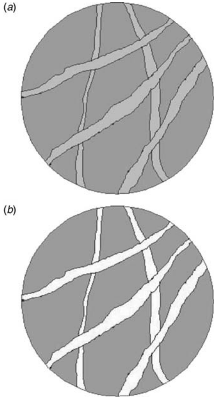
Figure 12.14. Spinodal decomposition pattern (a) with minor component leached out (b).
