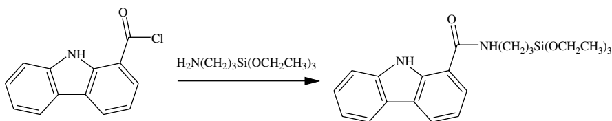
Figure 12.5. Carbazole-9-carbonyl chloride (CB) attached to 3-aminopropyltriethoxysilane.
